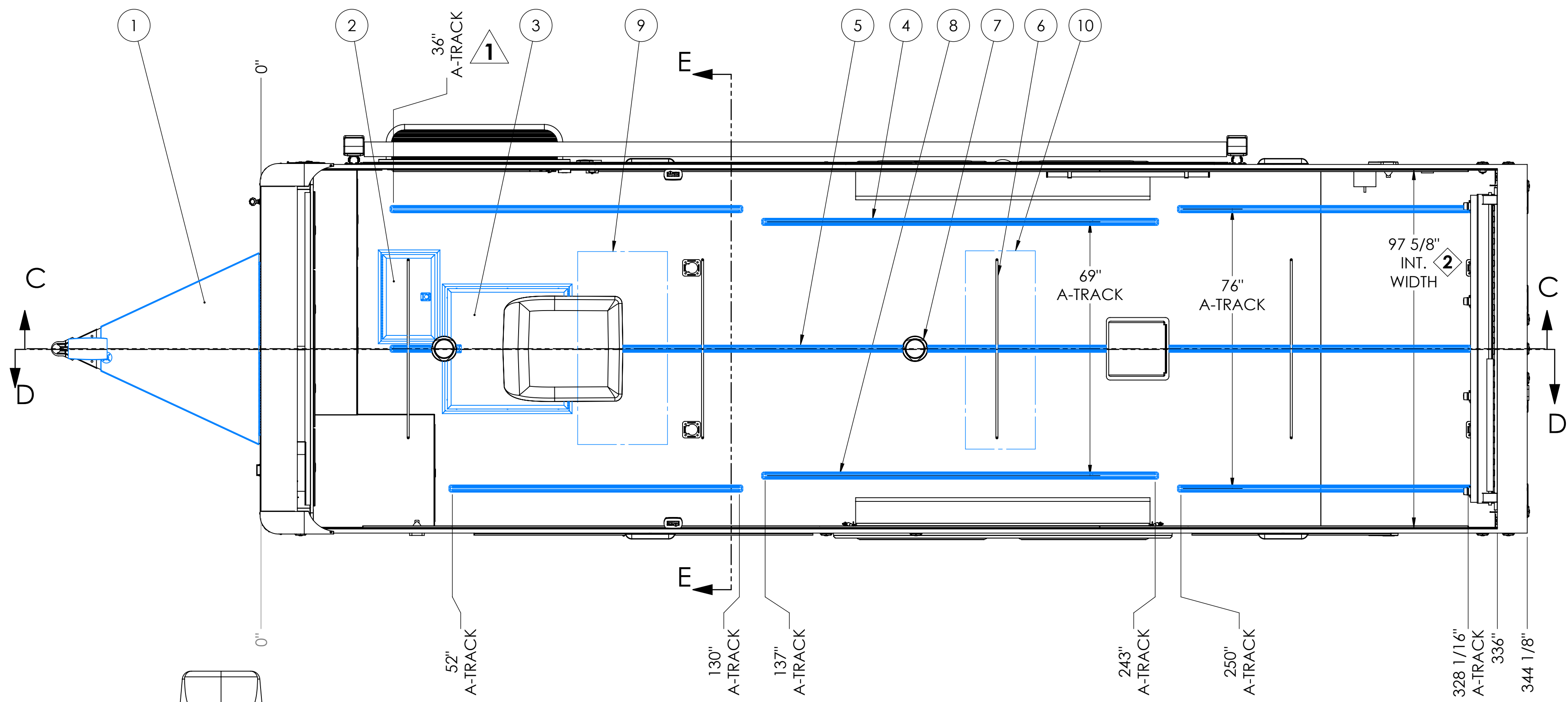
TOP VIEW POPULAR OPTIONS FLOOR LAYOUT
