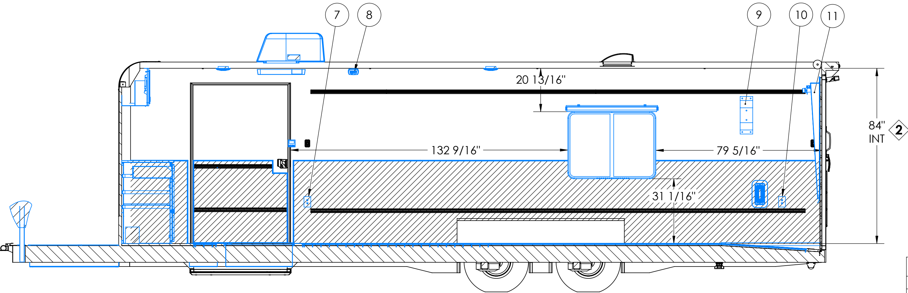
SECTION C-C SCALE 1 : 28
