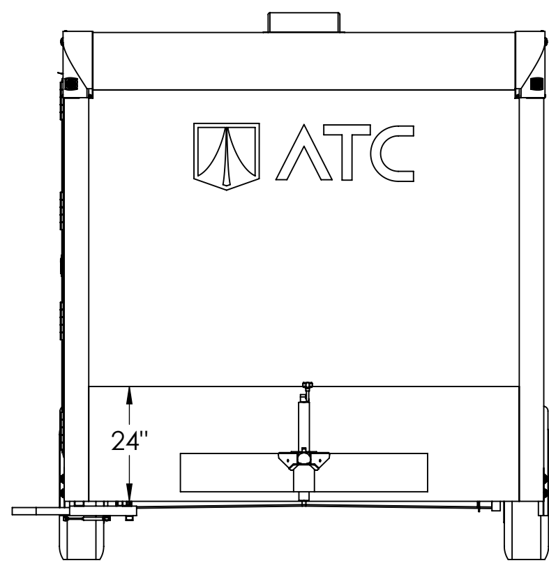
EXTERIOR FRONT VIEW
