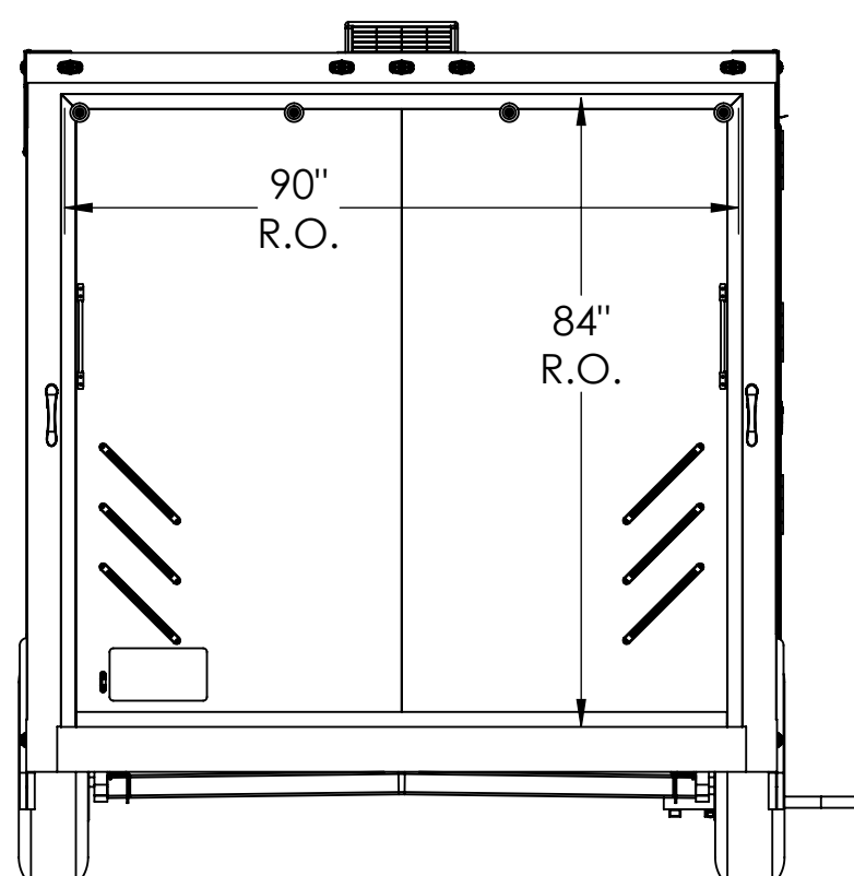
EXTERIOR REAR VIEW
